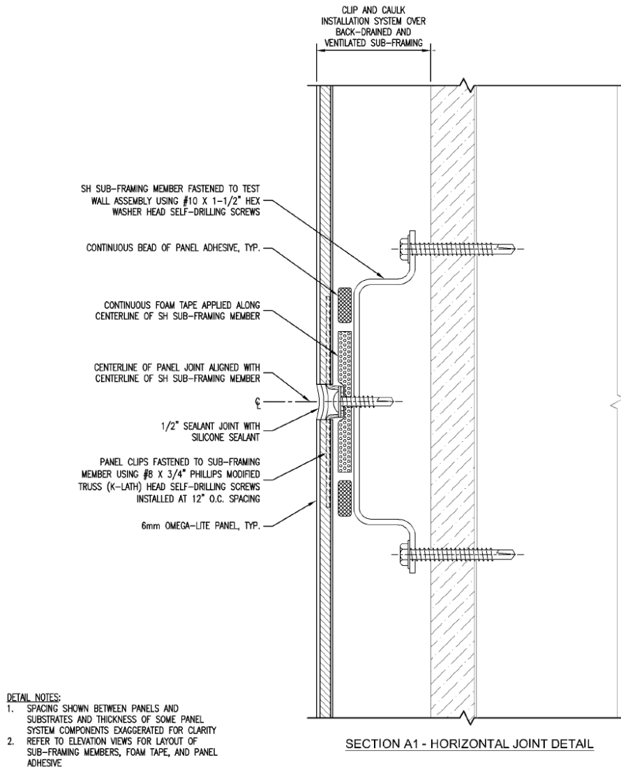
FIGURE 1—CLIP & CAULK INSTALLATION SYSTEM WITH HORIZONTAL LAYOUT OF BD&V SUB-FRAMING OVER GYPSUM SHEATHING
