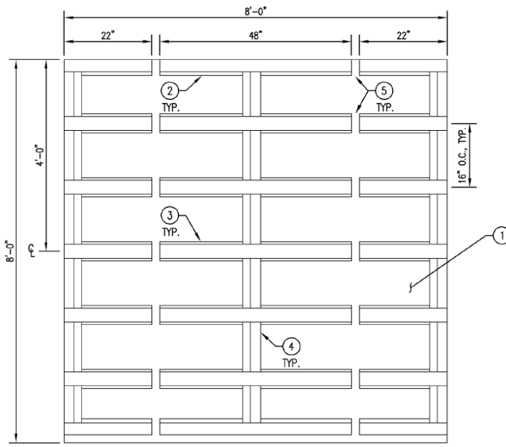
TEST WALL ASSEMBLY (AAMA 509) ELEVATION VIEW 1 - SUB-FRAMING LAYOUT
